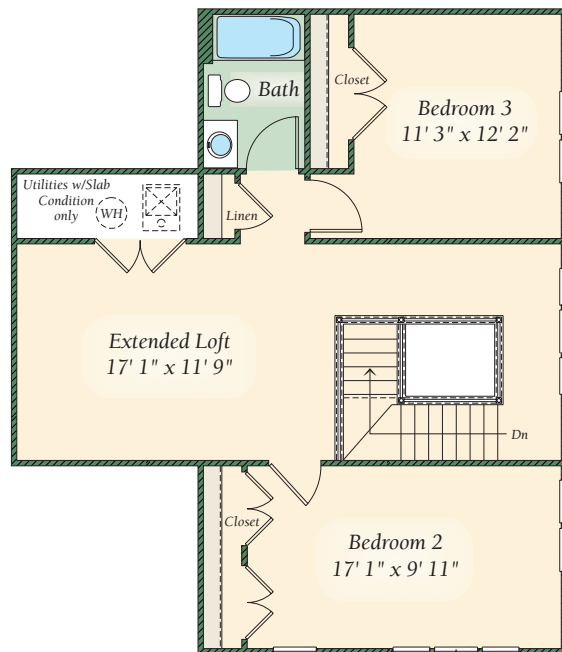
OPTIONAL SECOND FLOOR WITH EXTENDED LOFT
