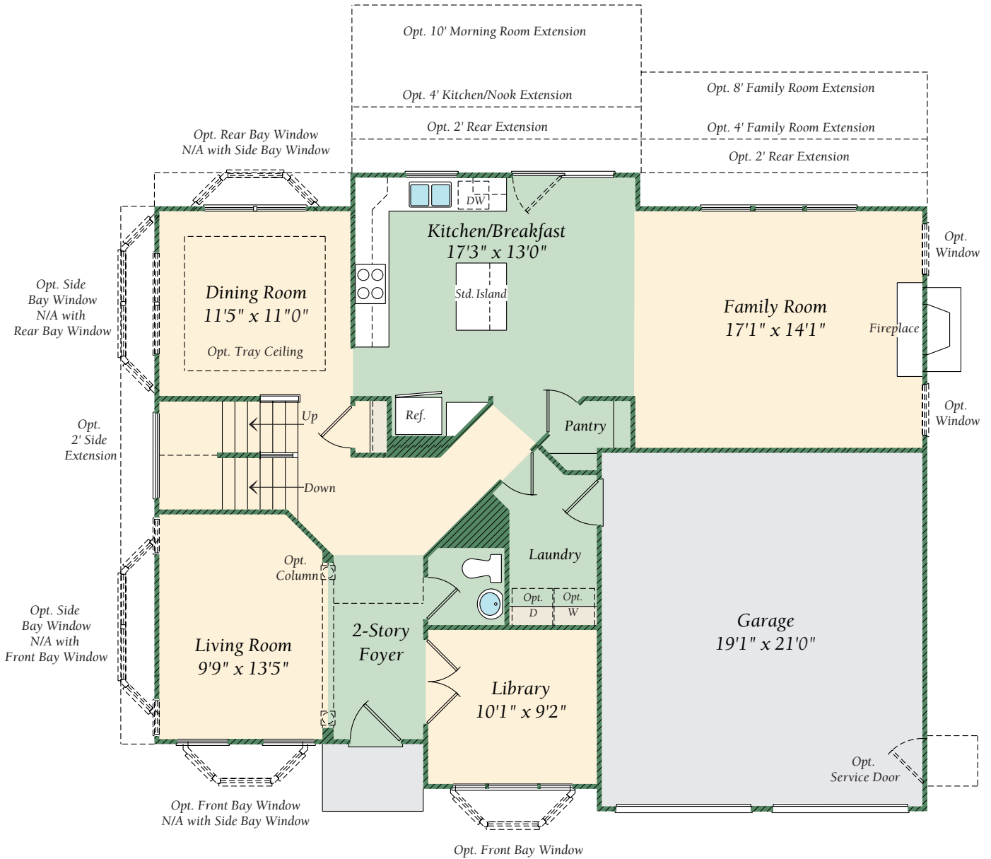
FIRST FLOOR
